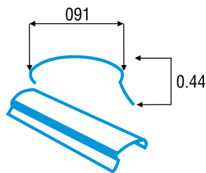
TDF Cleat
