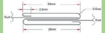
TRANSVERSE DUCT FLANGE (TDF)
