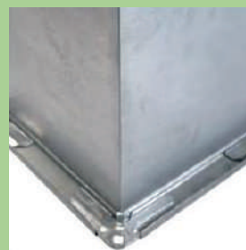
TRANSVERSE DUCT FLANGE (TDF)
