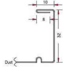
TRANSVERSE DUCT FLANGE (TDF)
