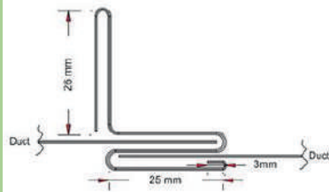
STANDING "S" Cleat
